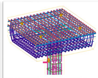
Railway Foot Over Bridge
